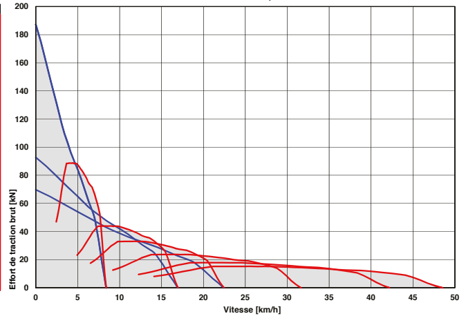
ADT, B20E 6X6 - Effort De Traction
